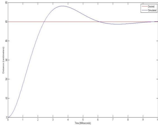
(a) Default PID Response
