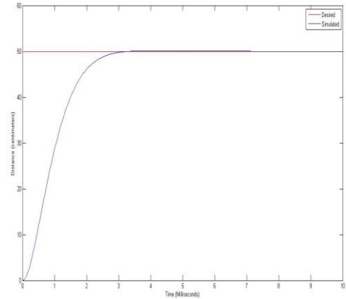
(b) Tuned PID Response
