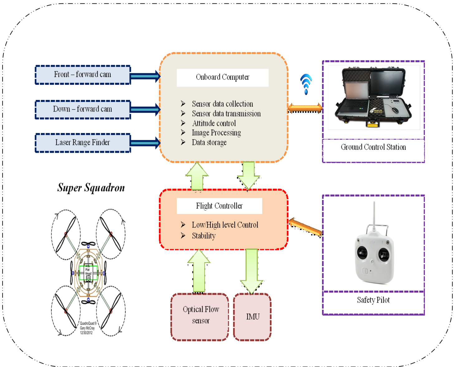
Figure 1. Overall system Architecture
